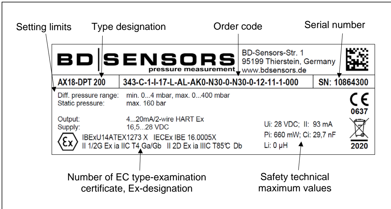
Fig. 1 Example of manufacturing label Ex ia
