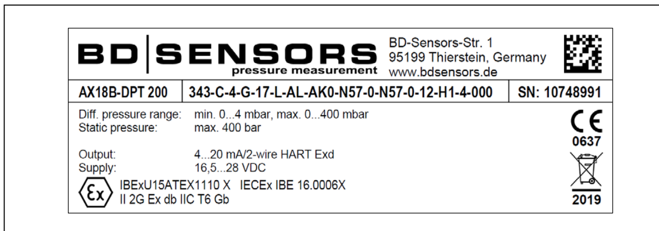
Fig. 2 Example of manufacturing label Ex d
